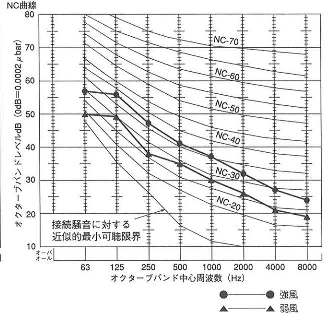
●YMEJ112・J140D-B1(200Pa)
