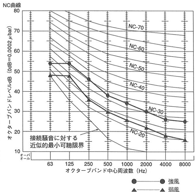
●YMEJ80D-B1(200Pa)
