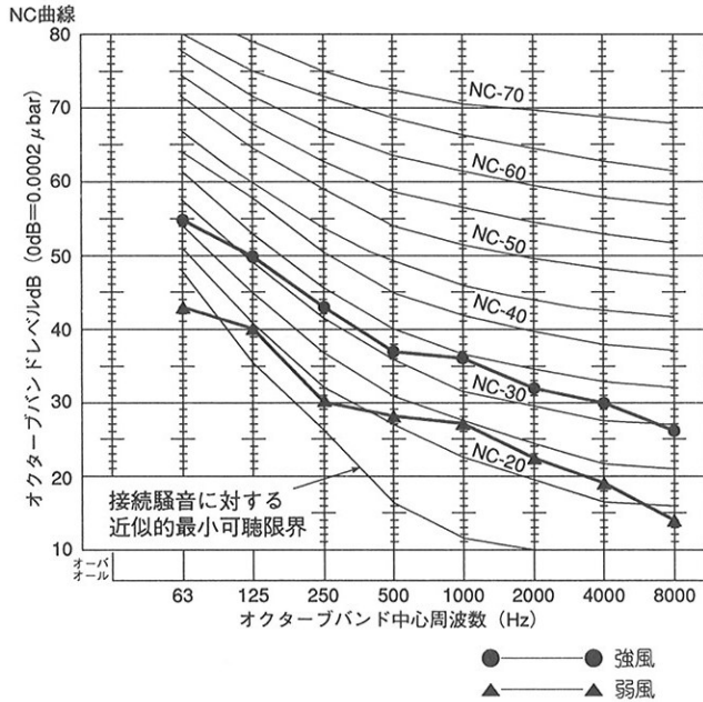
●YMEJ45D-B1(200Pa)
