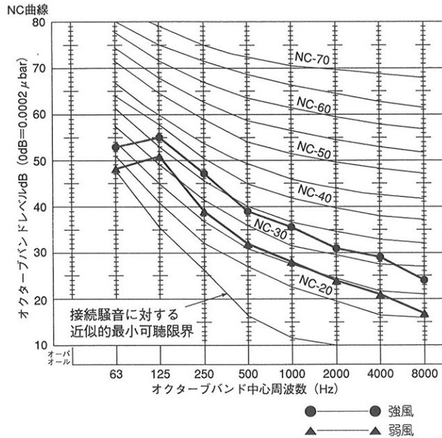
●YMEJ90D-B1(200Pa)
