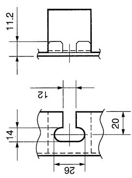
A (吊りボルト用穴詳細図)
