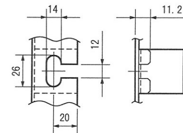
A (吊りボルト用穴詳細図)
